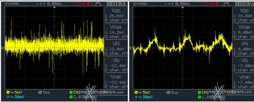
Low Frequency Ripple 3,3V @ 100%
