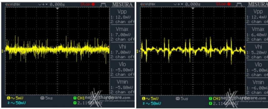
Low Frequency Ripple 3,3V @ 0%
