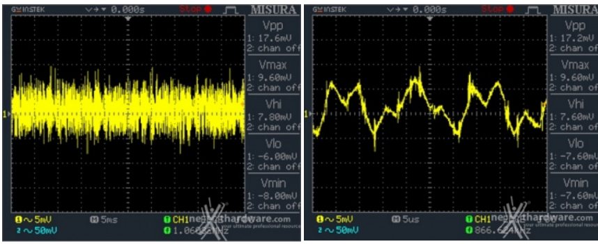
Low Frequency Ripple 5V @ 50%
