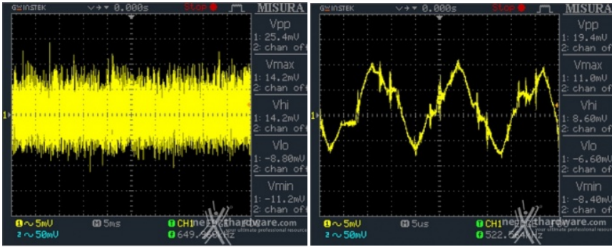
Low Frequency Ripple 5V @ 100%
