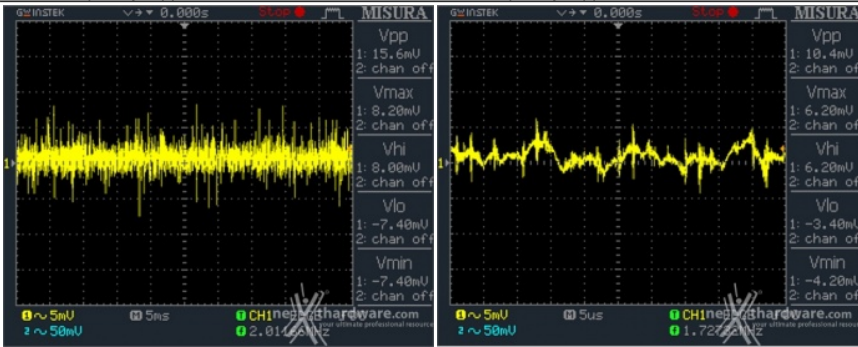
Low Frequency Ripple 3,3V @ 50%
