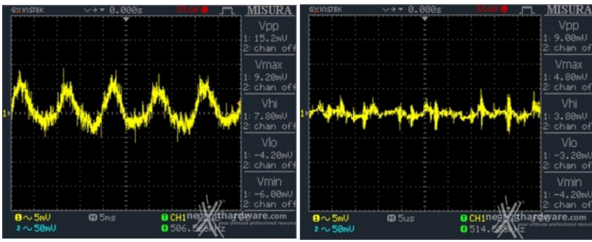
Low Frequency Ripple 12V @ 0%
