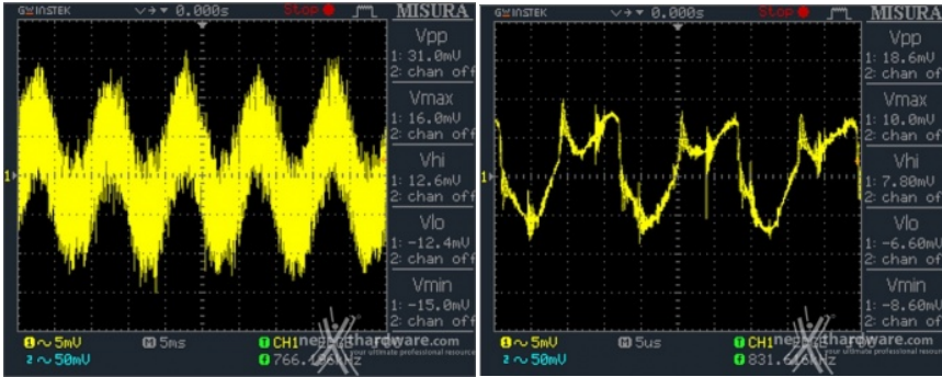
Low Frequency Ripple 12V @ 100%
