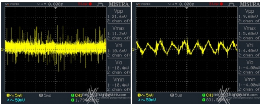
Low Frequency Ripple 5V @ 0%
