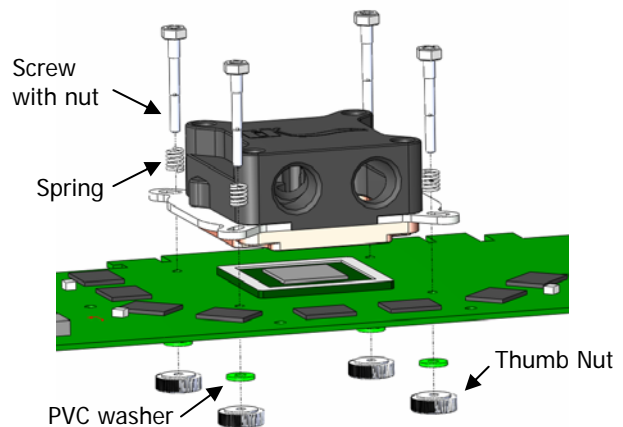
Picture 2: Properly installed water block
