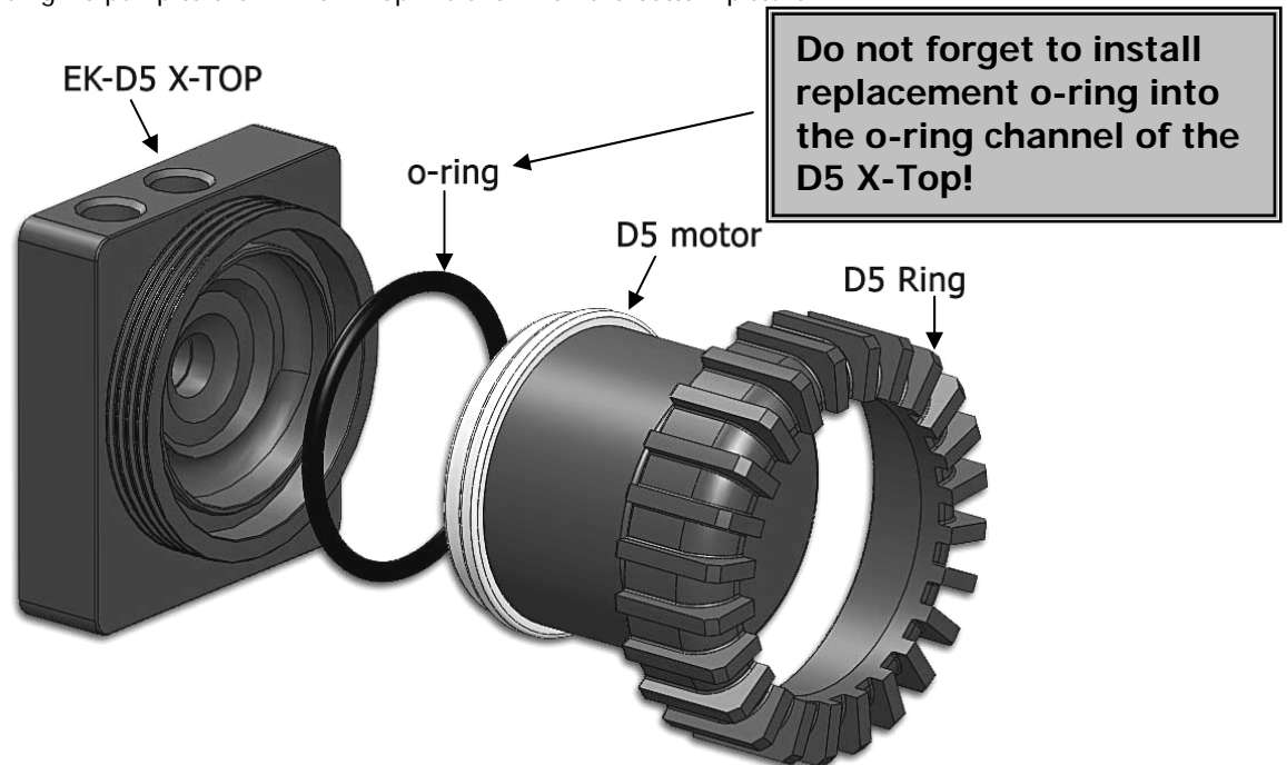
Picture 1: Assembling the EK-D5 X-Top to Laing D4/D5 Pump
