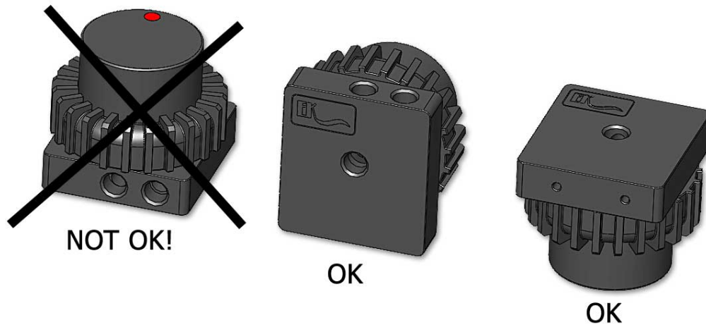
Picture 1: Assembling the EK-D5 X-Top to Laing D4/D5 Pump
