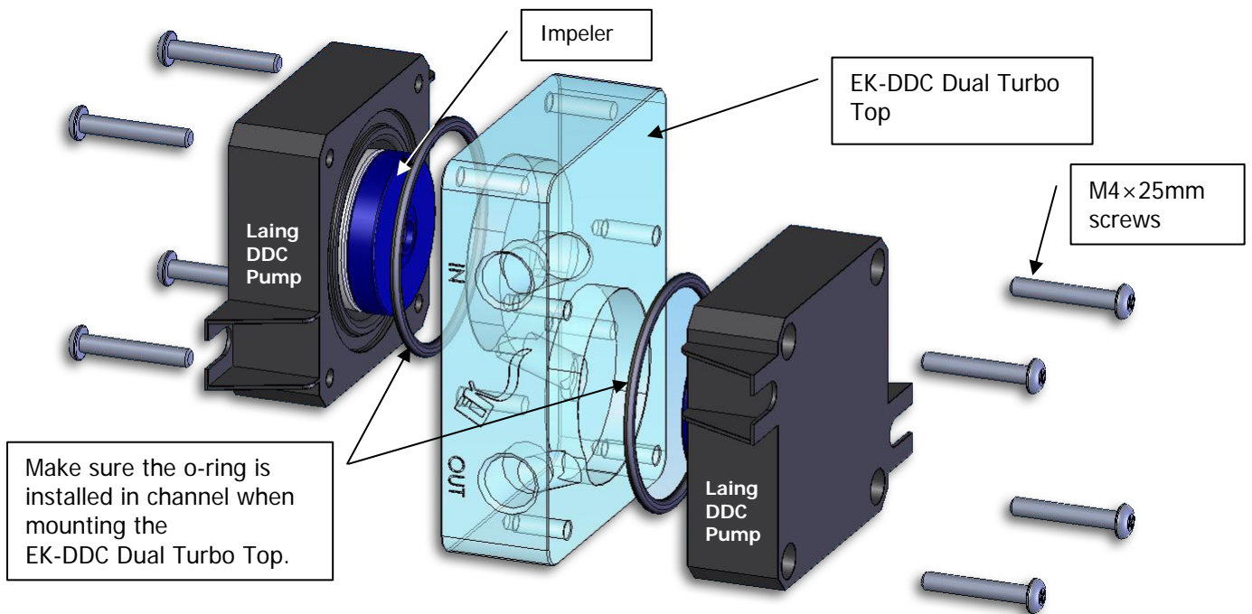
Picture 1: Installing the EK-DDC Dual Turbo Top
