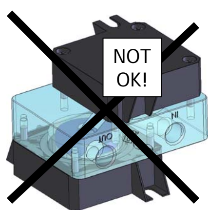
Picture 4: EK TOP installing NOT OK
